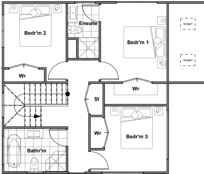
First floor - 67m 2 Note: excludes void area.
